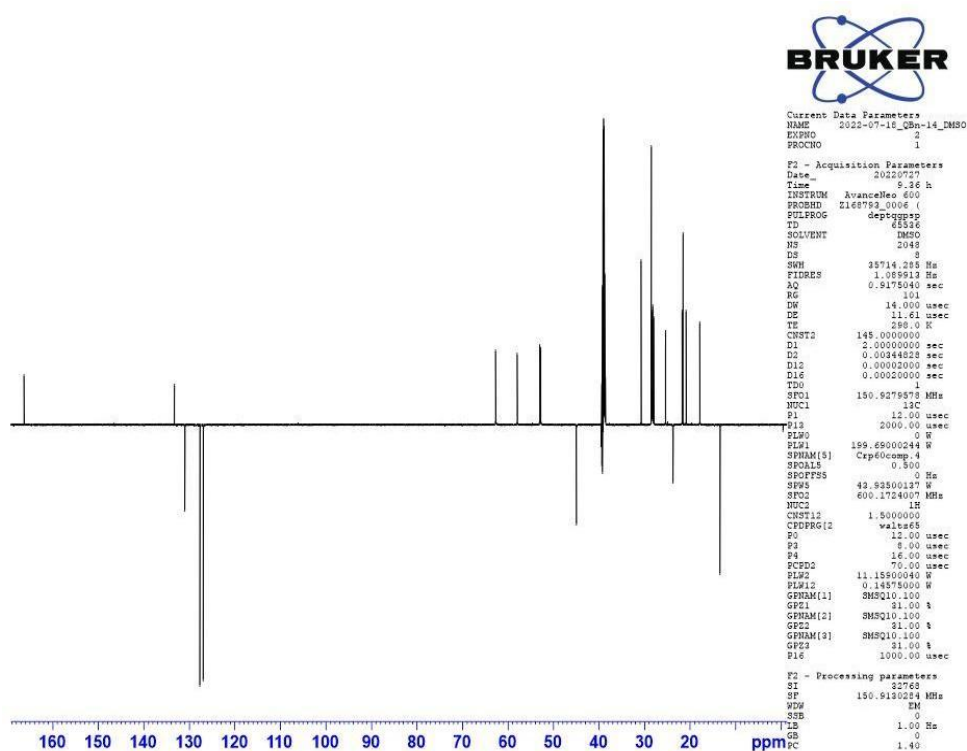
Slika 47. ^{13}\text{C} NMR spektar QBn- \text{C}_{14} .
