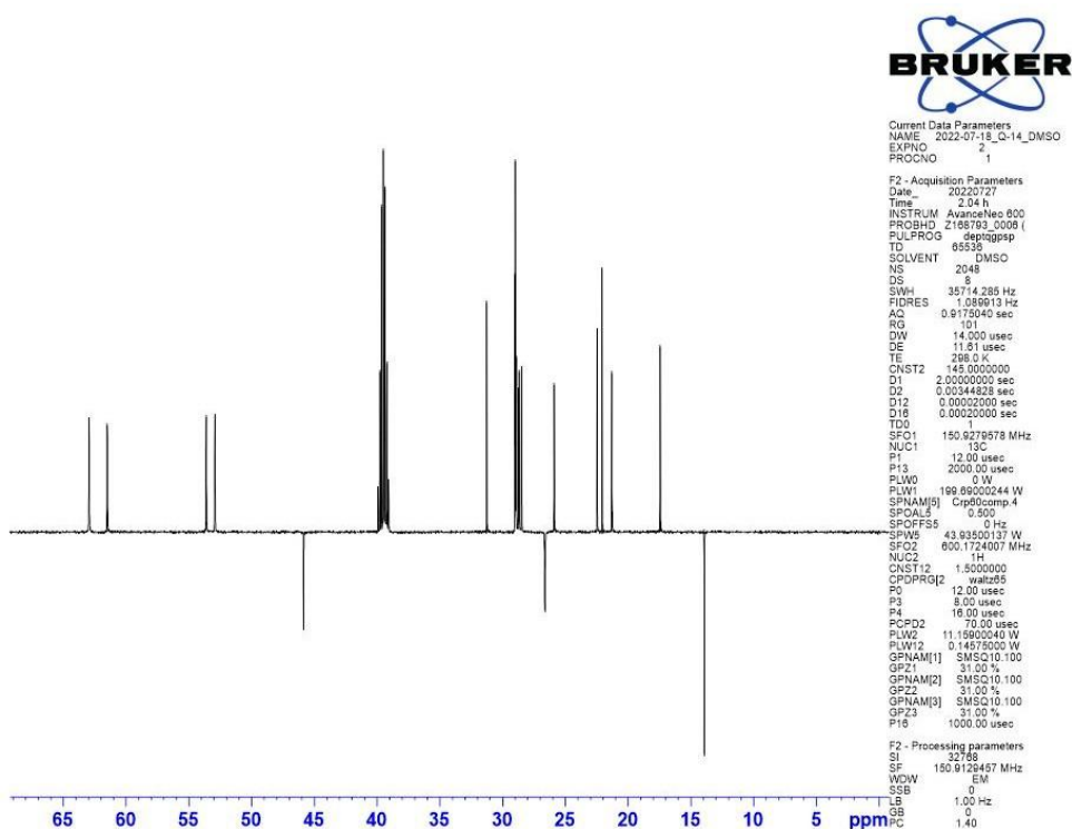
Slika 59. ^{13}\text{C} NMR spektar \text{QNH}_2\text{-C}_{14} .
