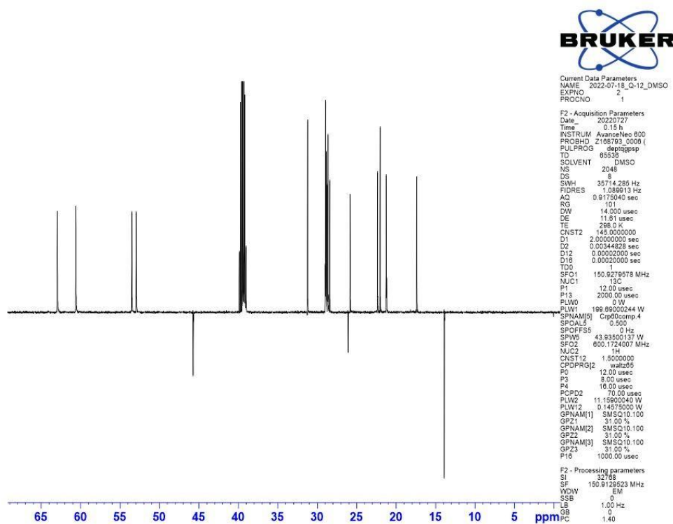
Slika 57. ^{13}\text{C} NMR spektar \text{QNH}_2\text{-C}_{12} .
