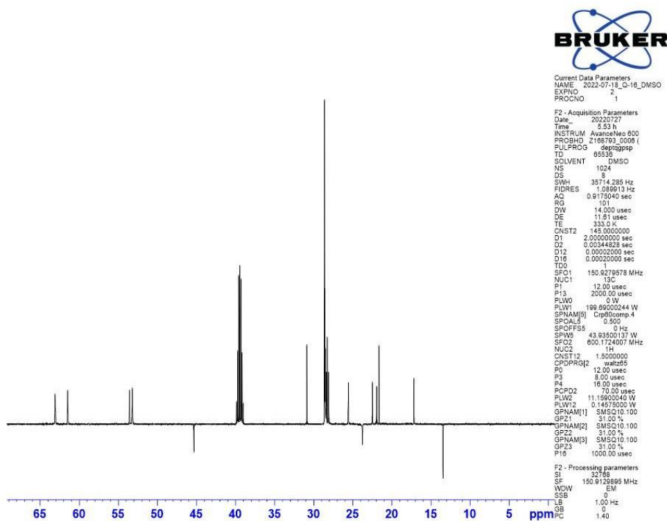
Slika 61. ^{13}\text{C} NMR spektar \text{QNH}_2\text{-C}_{16} .
