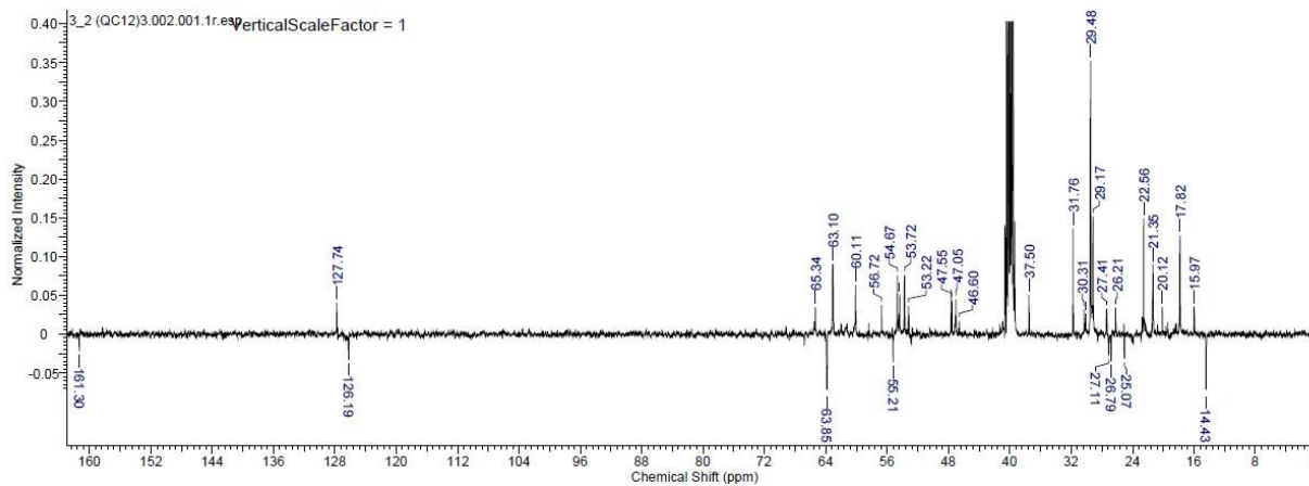
Slika 71. ^{13}\text{C} NMR 2(QC 12 ) 3 .
