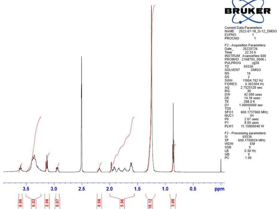
Slika 56. ^1\text{H} NMR spektar \text{QNH}_2\text{-C}_{12} .
