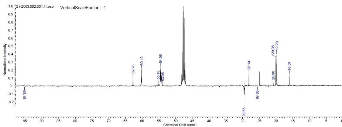
Slika 67. ^{13}\text{C} NMR 2(\text{QO})_3 .
