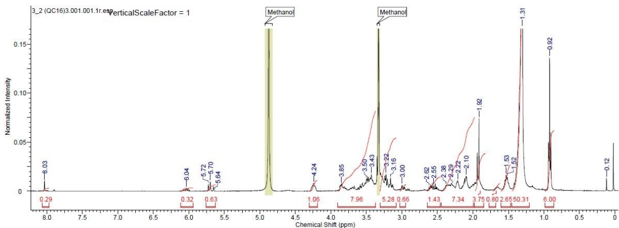
Slika 74. ^1\text{H} NMR 2(\text{QC}_{16})_3 .
