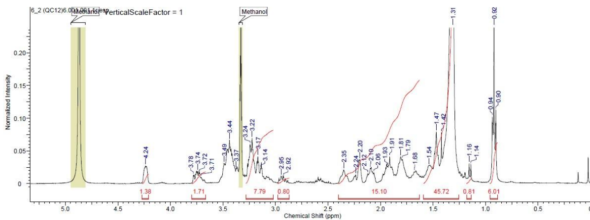
Slika 82. ^1\text{H} NMR 2(QC 12 ) 6 .
