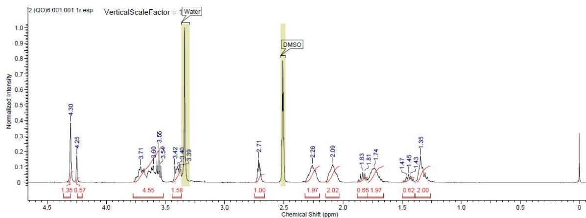
Slika 68. ^1\text{H} NMR spektar 2(\text{QO})_6
