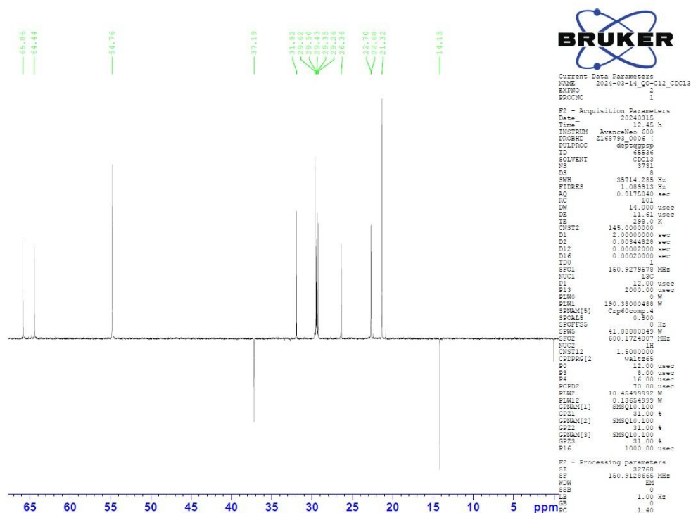
Slika 62. ^{13}\text{C} NMR spektar QO- \text{C}_{12} .
