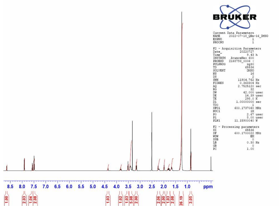
Slika 48. ^1\text{H} NMR spektar QBn- \text{C}_{16} .
