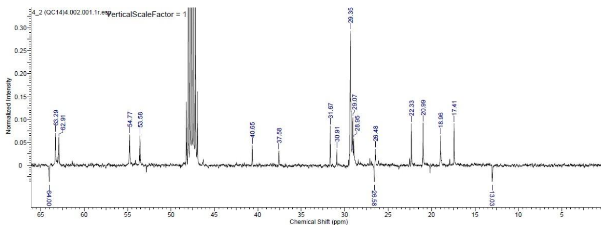
Slika 79. ^{13}\text{C} NMR 2(QC 14 ) 4 .
