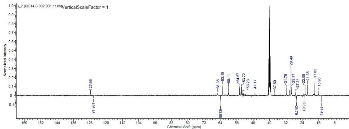
Slika 73. ^{13}\text{C} NMR 2(\text{QC}_{14})_3 .
