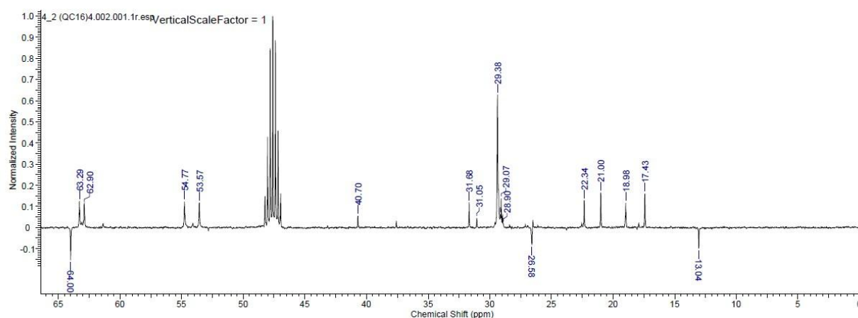
Slika 81. ^{13}\text{C} NMR 2(QC 16 ) 4 .
